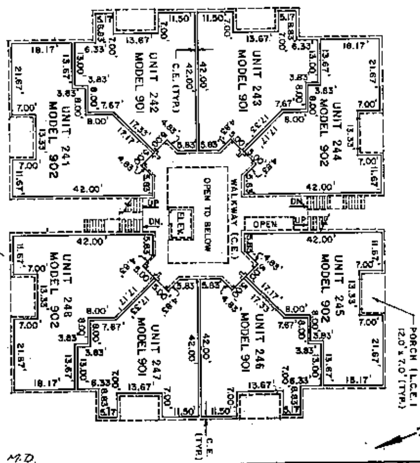
SECOND FLOOR 3411 MIN. UPPER LIMIT OF UNITS 33-95 ELEV. (N.G.V.D.) MIN. LOWER LIMIT OF UNITS 25-70 ELEV. (N.G.V.D.) 25-93
