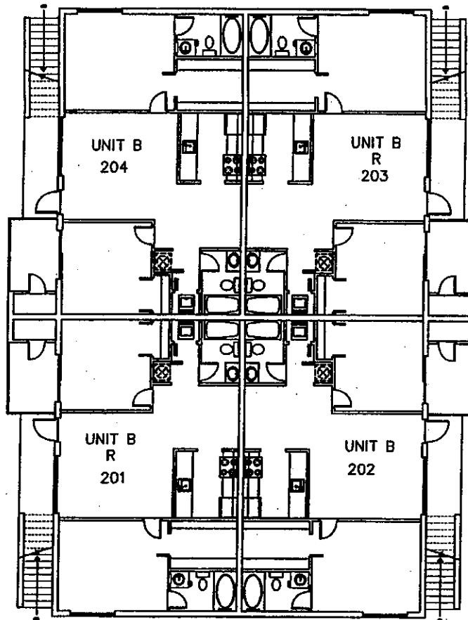
2ND FLOOR BUILDING #10
