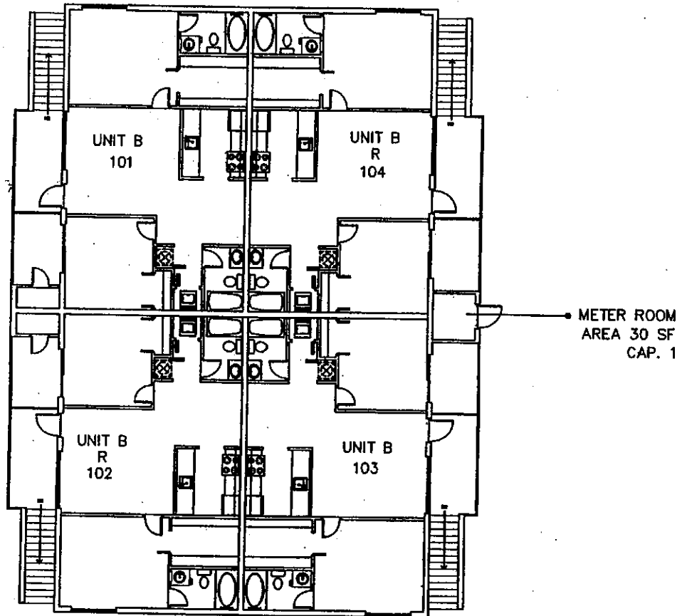
GROUND FLOOR BUILDING #16
