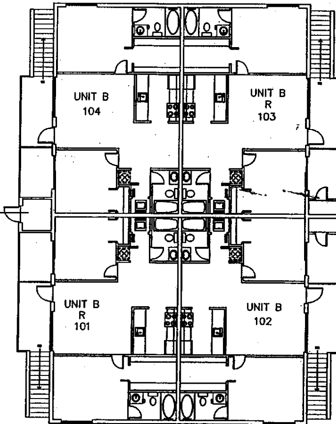
GROUND FLOOR BUILDING #14
