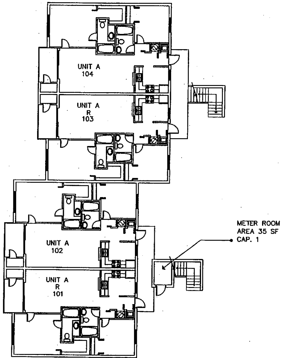
GROUND FLOOR BUILDING #8
