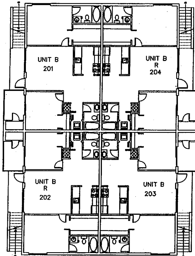
2ND FLOOR BUILDING #18
