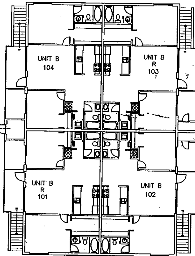
GROUND FLOOR BUILDING #10
