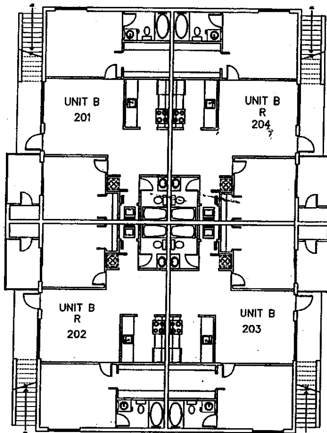
2ND FLOOR BUILDING #16
