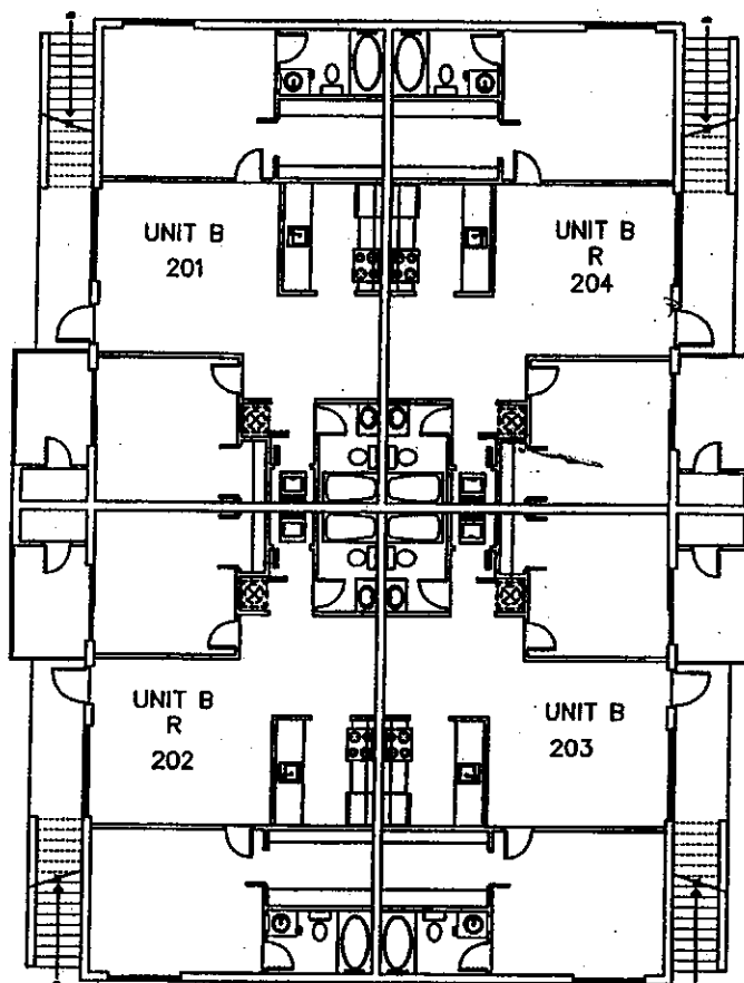
2ND FLOOR BUILDING #20
