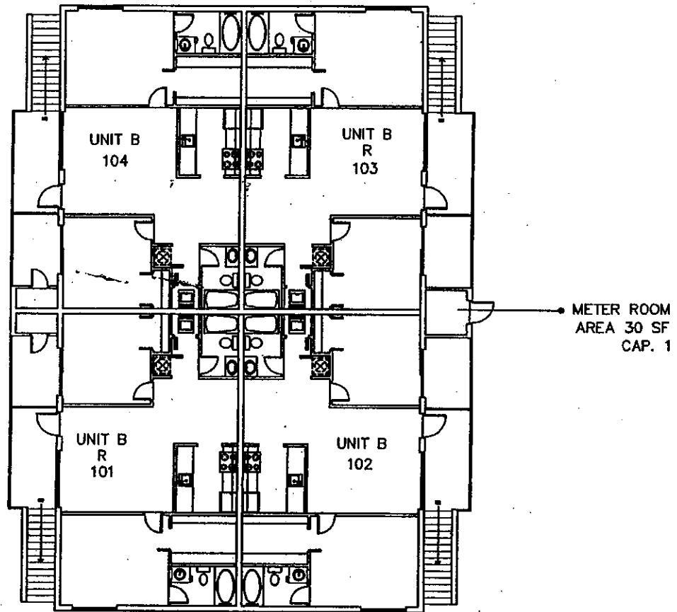
GROUND FLOOR BUILDING #15
