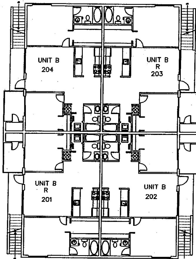
2ND FLOOR BUILDING #19
