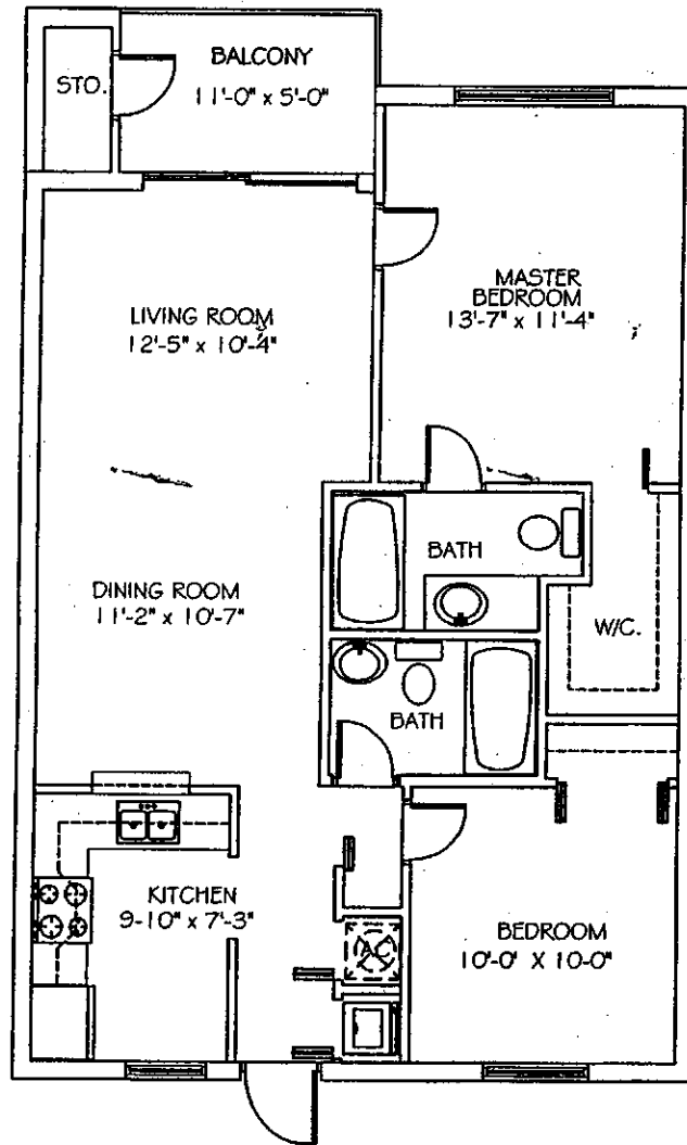
UNIT B 2 BEDROOMS / 2 BATH SCALE \frac{1}{8} = 1'-0
