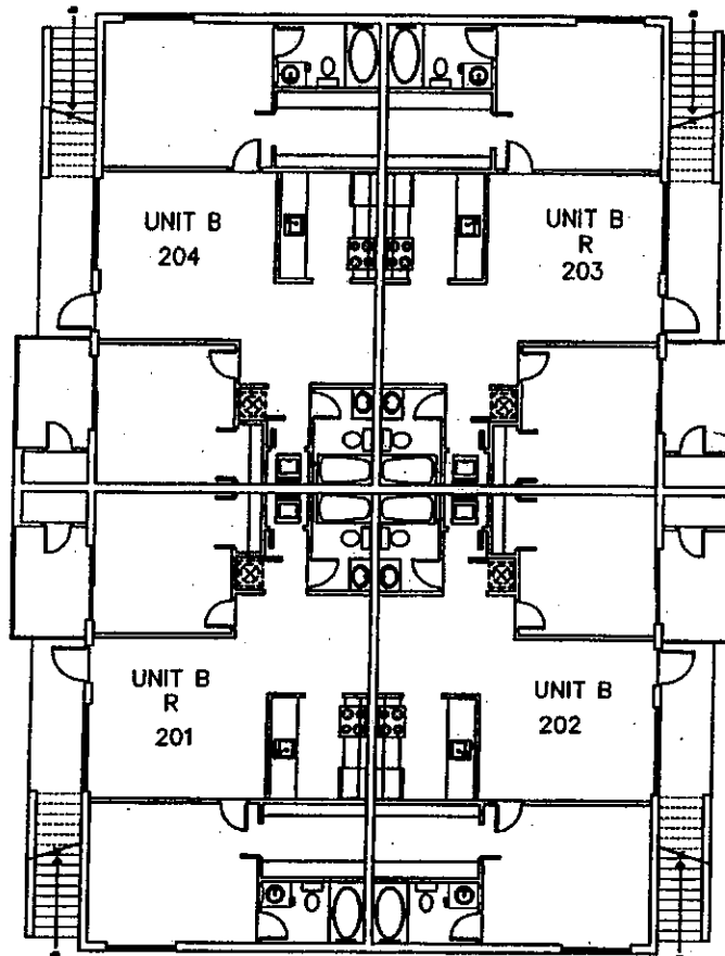
2ND FLOOR BUILDING #15
