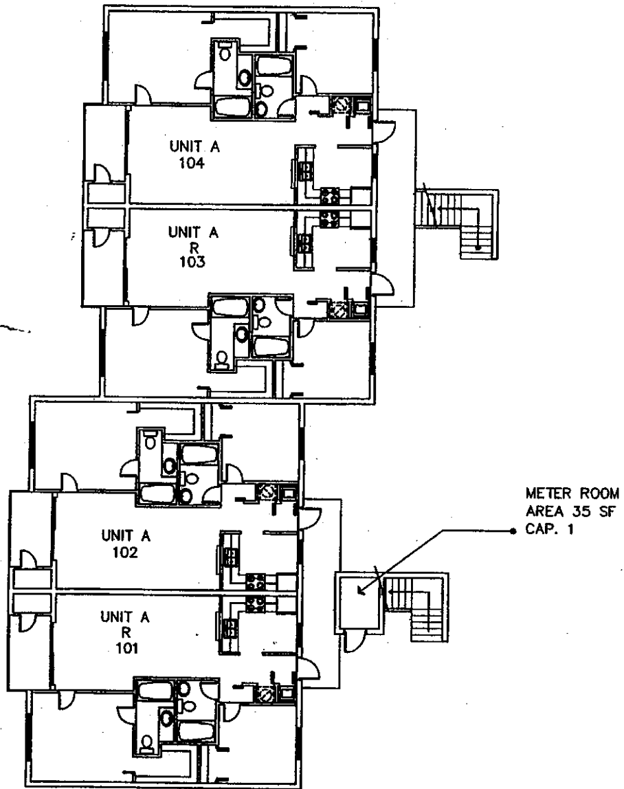
GROUND FLOOR BUILDING #7
