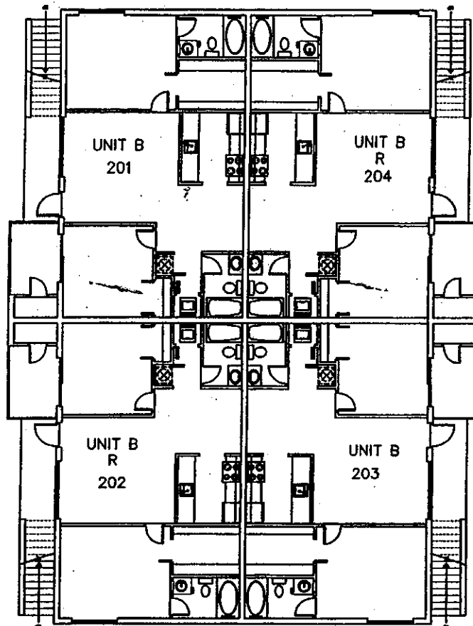
2ND FLOOR BUILDING #21
