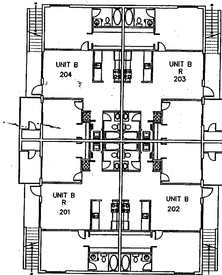
2ND FLOOR BUILDING #17
