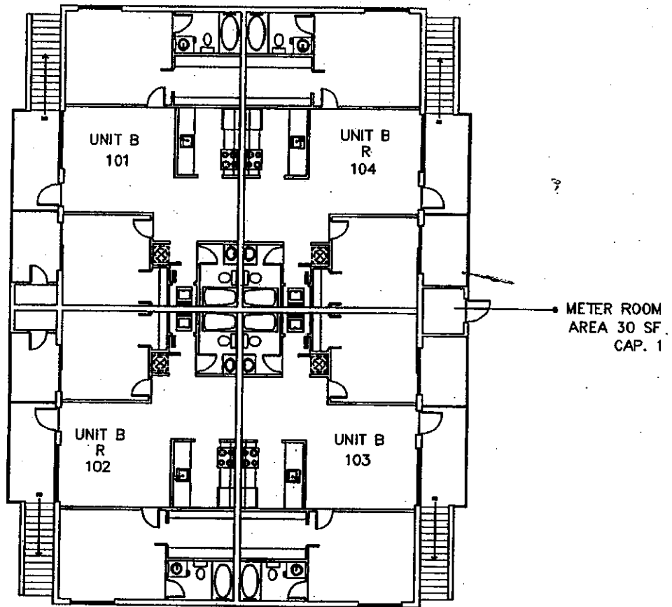
GROUND FLOOR BUILDING #22
