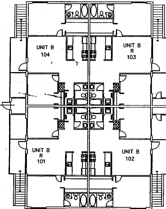
GROUND FLOOR BUILDING #11
