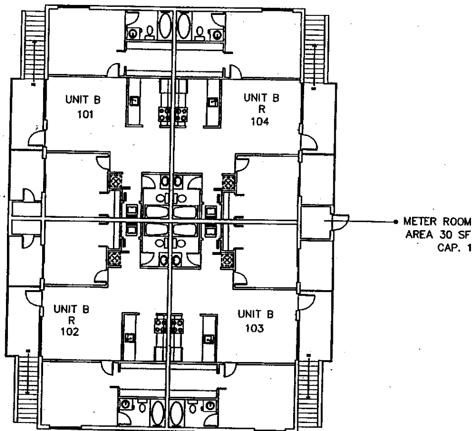
GROUND FLOOR BUILDING #21
