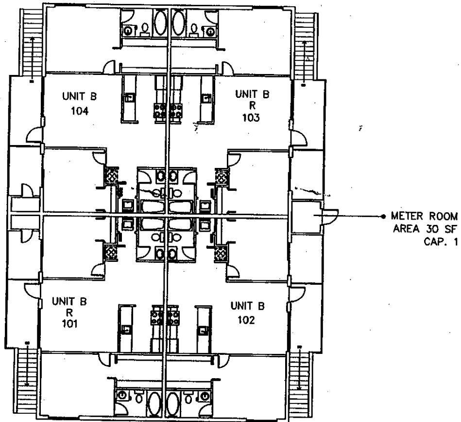
GROUND FLOOR BUILDING #19
