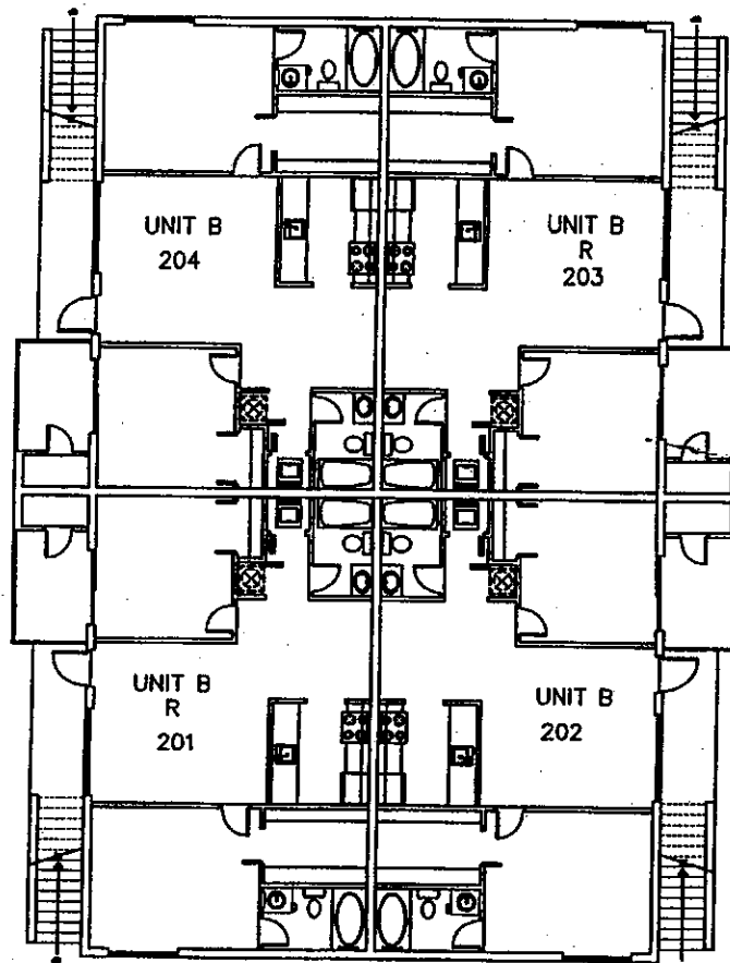
2ND FLOOR BUILDING #11
