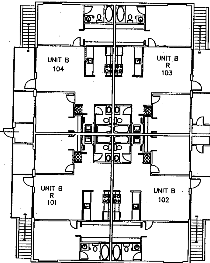
GROUND FLOOR BUILDING #17
